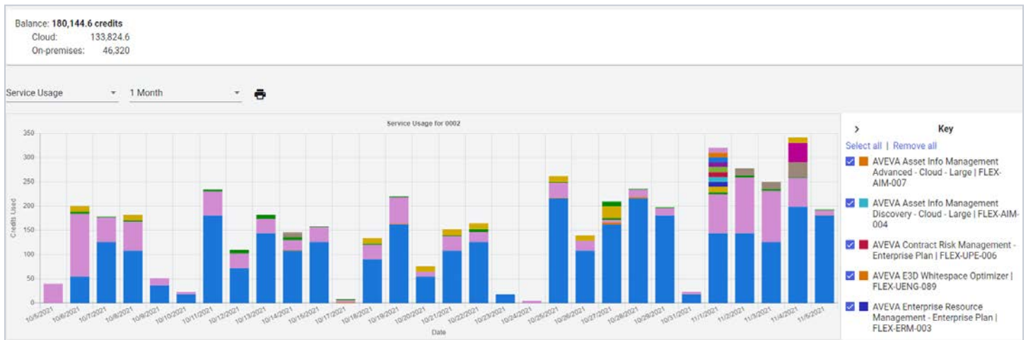
Credit consumption by service
